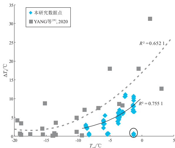
图 7 流体包裹体显微测温实验 T_{m0} 与 \Delta T_h 交会图 Fig.7 Cross plots of T_{m0} and \Delta T_h values of fluid inclusion microthermometric measurement
