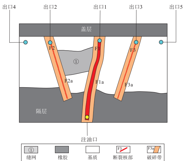
图 6 塔里木盆地顺北地区 S53-2 井设计模型 Fig.6 Design model of well S53-2 in Shunbei area, Tarim Basin
